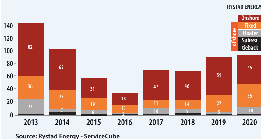
Figure 2: EPCI global greenfield contract awards worldwide are on the rise.
